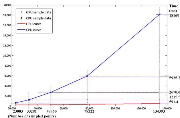
Fig. 7 Comparison of BP on CPU and GPU. The time cost of CPU implementation increases fast while the sampled points increase
